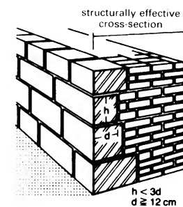
⑨ Mixed masonry with structurally effective cross-section
